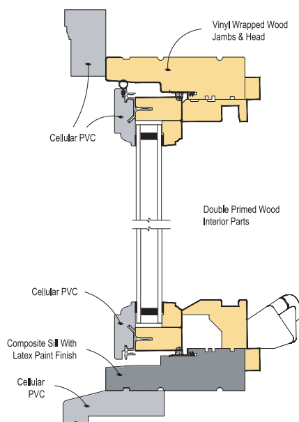
Legend Casement
