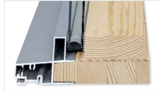
Low Profile Direct Set
