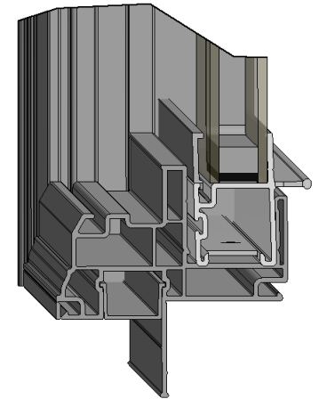
Single Hung
