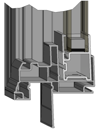
Slider
