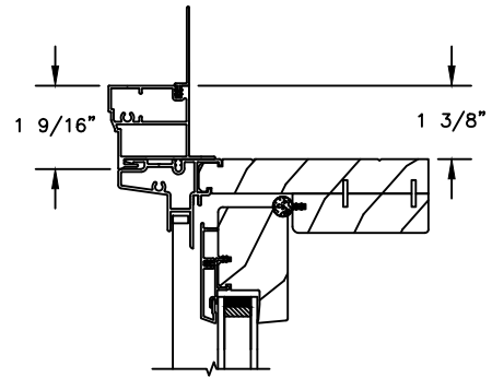
HEAD JAMB WITH CLAD SQUARE BRICKMOULD CASING
