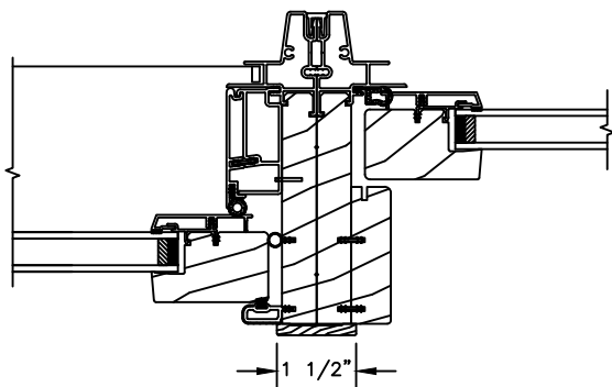
VERTICAL MULLION OPERATOR/OPERATOR
