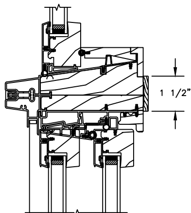
HORIZONTAL MULLION TRANSOM/OPERATOR
