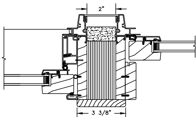
VERTICAL MULLION WITH 2" SPREAD MULL ADDITIONAL WIDTHS INCLUDE: 1", 2", 2 1/2", 3", & 4"
