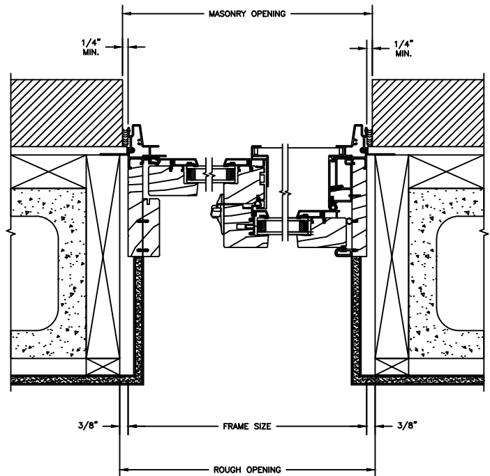
JAMBS 8" CONCRETE BLOCK WALL WITH BRICK VENEER
