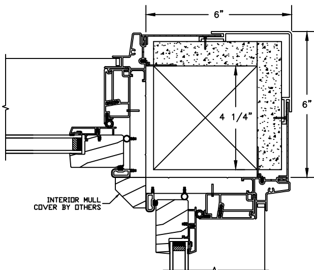
90° MULLION OPERATOR/OPERATOR (ONLY USED WITH 4 9/16" JAMB & 3 1/4" FRAME EXPANDER)
